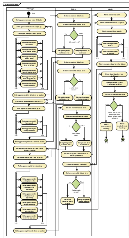
Gambar 3. Activity Diagram
