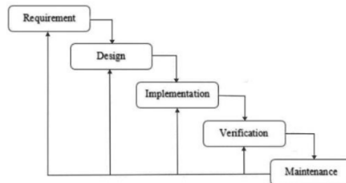
Gambar 1. Model SDLC Waterfall
