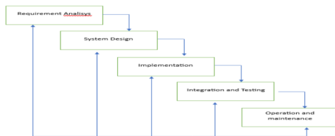
Gambar 1. Tahapan Waterfall
