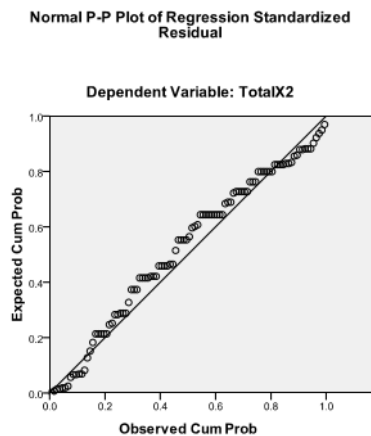
Gambar 1. grafik normal p-plot ( M = a + b_1X_1 + e )
